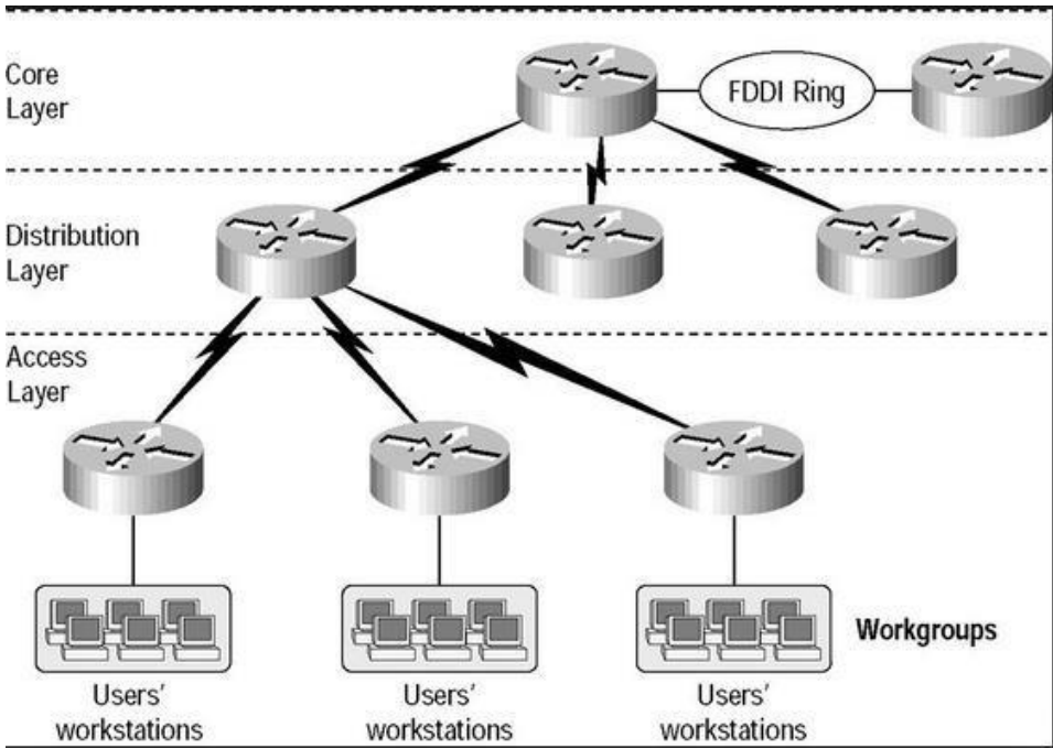
Gambar 30 Three Layered Model Hierarchical via tech-faq.com
