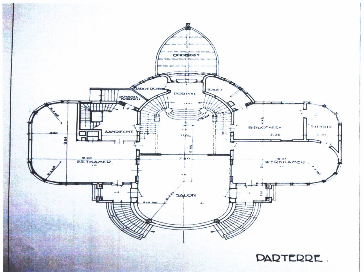
Gambar 10. Site Plan asli Villa Isola beserta denah lantai dasar. Sumber: Lemei, W. (1934)
